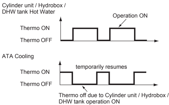
Operating state when ATA Cooling and hot water supply operations are requested at the same time
